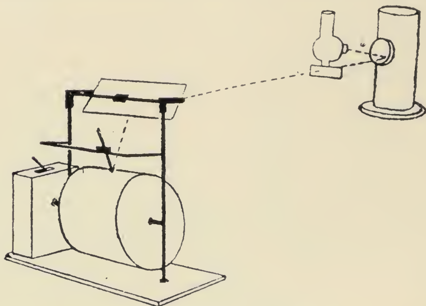
FIG. 100. Response Recorder.
